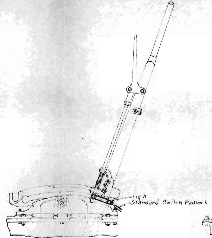
APPLICATION OF LATCH LOCK SHACKLE FIG A ON SAXBY & FARMER INTERLOCKING MACHINE LEVER
