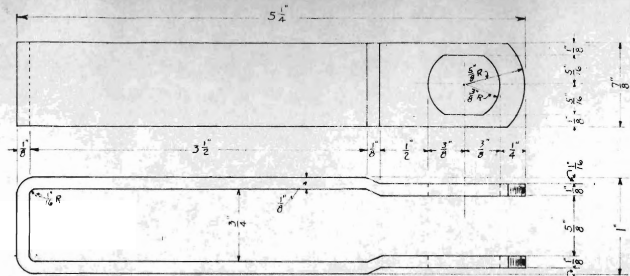
FIG. A - LATCH LOCK SHACKLE FOR SAXBY & FARMER MACHINE Scale - Full Size
