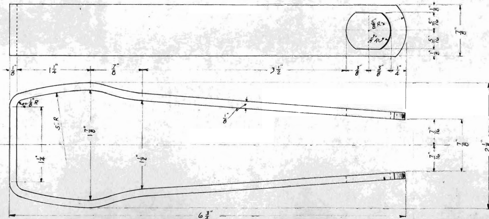
FIG. B - LATCH LOCK SHACKLE FOR STYLE "A" MACHINE Scale - Full Size
