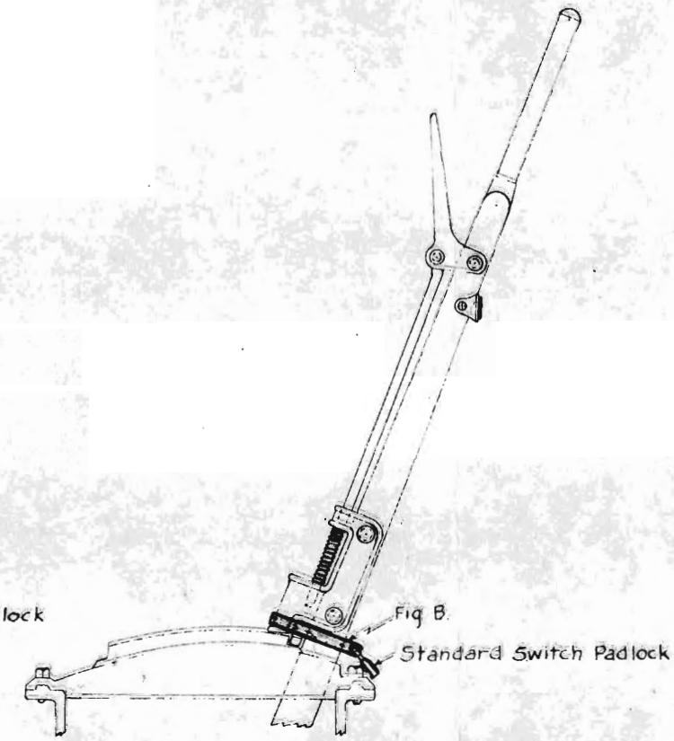
APPLICATION OF LATCH LOCK SHACKLE FIG B ON STYLE "A" INTERLOCKING MACHINE LEVER
