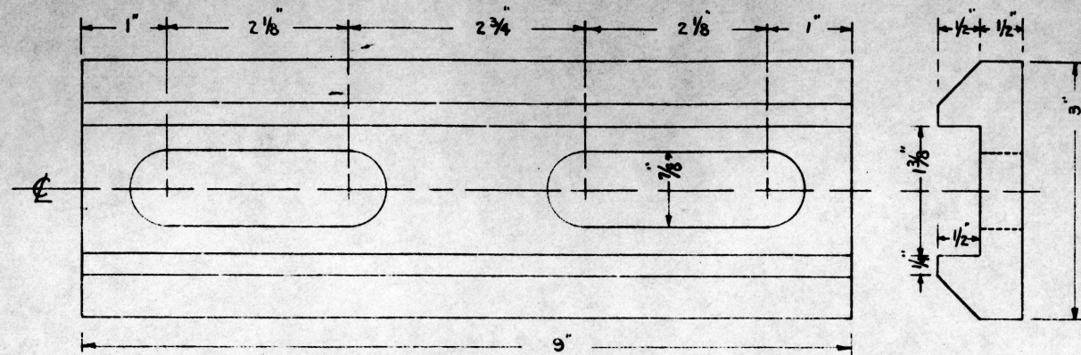
FIG. "A" WASHER PLATE (CAST IRON) PAT. NO. R 5081
