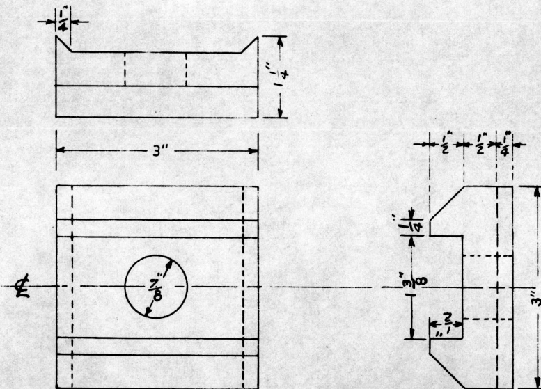
FIG. B WASHER PLATE (CAST IRON) PAT. NO. R-5266
