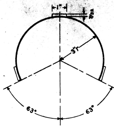
HOOD FOR A.&W. #1184 LAMP (22 GAUGE SHEET METAL) "PAINT DULL BLACK"
