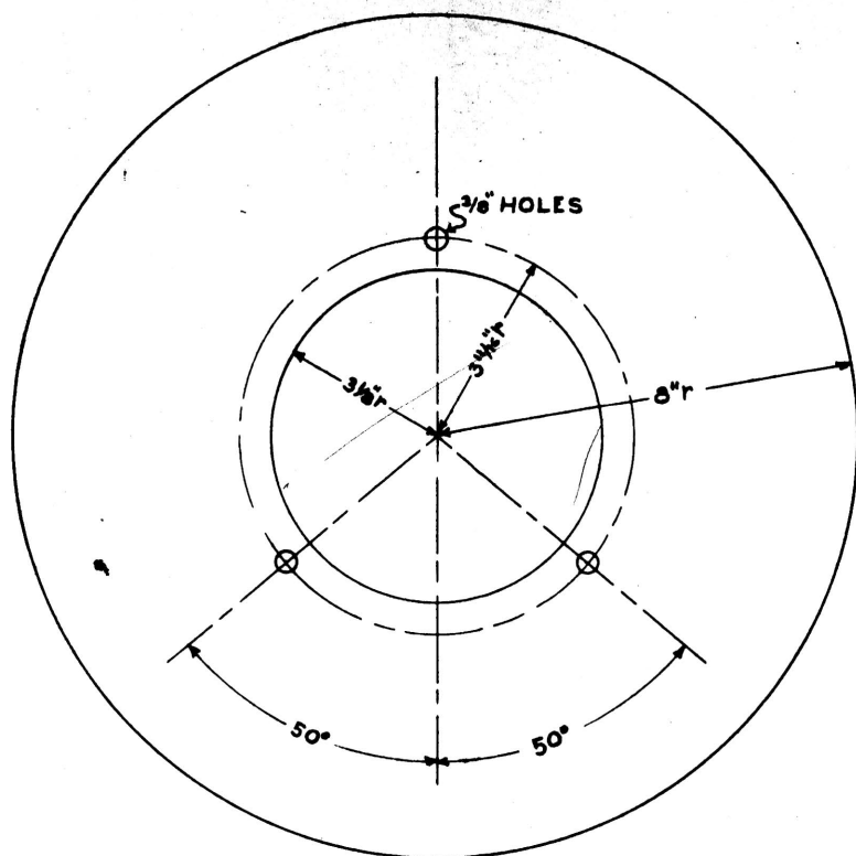
BACKGROUND FOR A.&W. #1184 LAMP (16 GAUGE SHEET METAL) "PAINT DULL BLACK"
