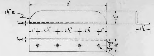
COVER ANGLE
