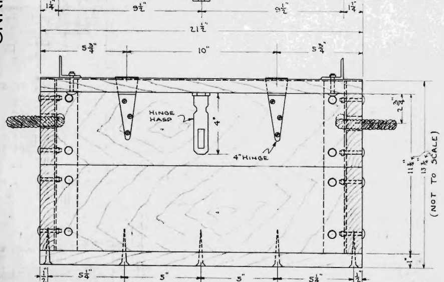
BACK VIEW
