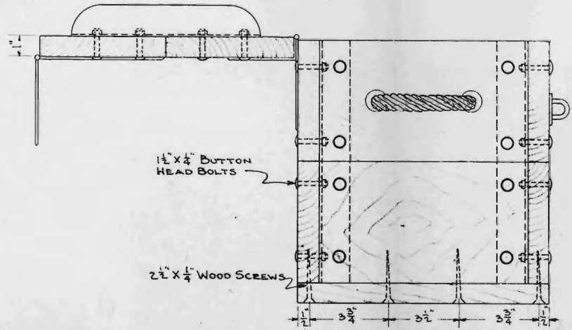
END VIEW
