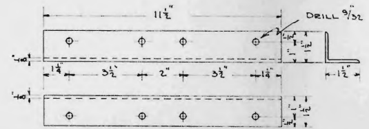
CORNER ANGLE
