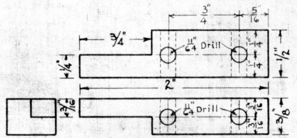
FIG. B SWITCH POINT GAUGE (COLD ROLLED STEEL) ALL SIDES FINISHED TO DIMENSIONS
