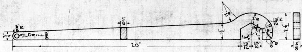
FIG. A SWITCH ADJUSTING WRENCH (MILD STEEL)
