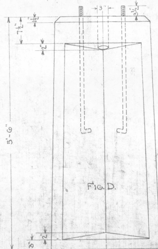
FOUNDATION FOR GROUND MAST SIGNAL-SEMAPHORE TYPE
