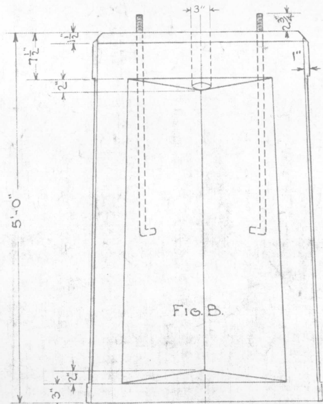
FOUNDATION FOR CASE SIGNAL LIGHT TYPE
