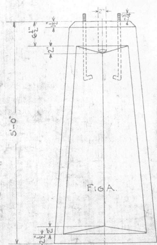
FOUNDATION FOR CABLE POST
