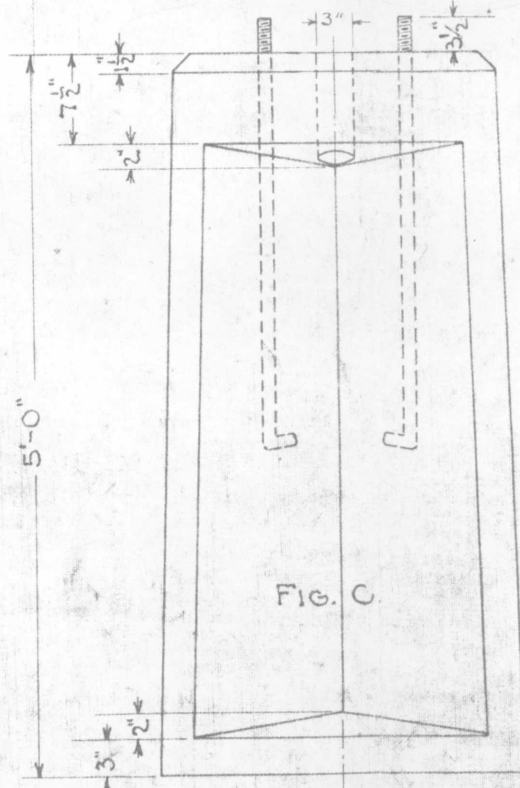
FOUNDATION FOR GROUND MAST SIGNAL LIGHT TYPE
