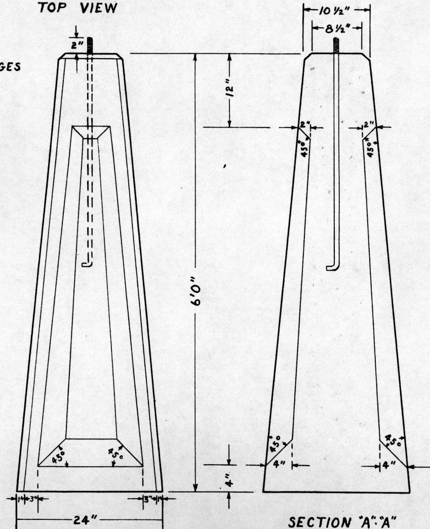
SIDE VIEW
